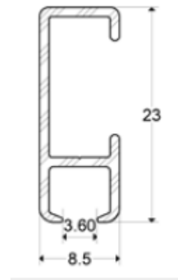
Profilmasse in mm
